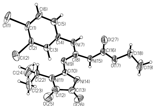
Figure 1. Thermal ellipsoid plot of crystalline 3a , N -(3,4-dichlorophenyl)- N' -ethylcarbonyl- N'' -(1-isopropyl-4,5-dioxo-imidazolidin-2-ylidene)-guanidine, showing the atom numbering scheme used for the X-ray crystallographic data. Atoms N7, C8, N9, C10, N11, C12, C13, N14, N15, C16, O17, O25, O26, and O27 are essentially co-planar with atom N7 showing the largest deviation (0.13 Å) off a least-squares plane through these atoms. The phenyl ring is angled such that the C3–C4–N7–C8 torsion angle is 52.8°. The crystal structure contained only intramolecular hydrogen bonds, between N7–H7 and O27 and N15–H15 and N14. The N7–H7···O27 angle is 131.1°, H7···O27 distance is 2.029 Å, and N7···O27 distance is 2.674 Å. The N15–H15···N14 angle is 139.8°, H15···N14 distance is 1.879 Å, and N15···N14 distance is 2.660 Å.
