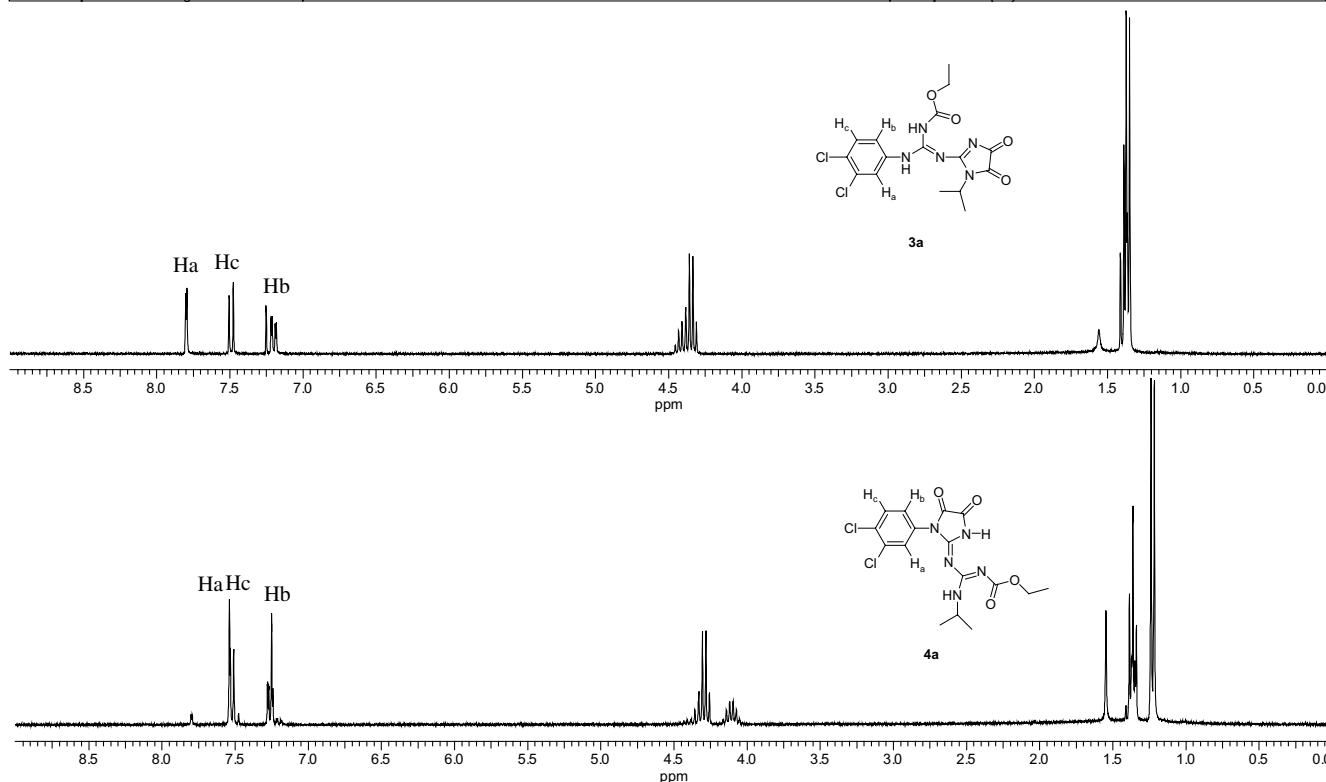
Figure 3. NMR spectrum of 3a and 4a .
