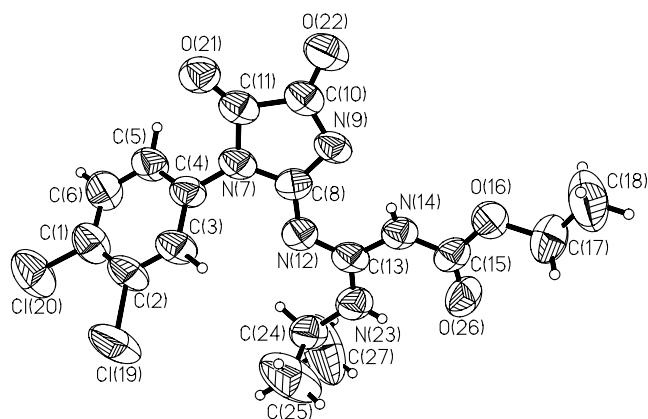
Figure 2. Thermal ellipsoid plot of crystalline 4a , N -[1-(3,4-dichlorophenyl)-4,5-dioxo-imidazolidin-2-ylidene]- N' -isopropyl- N'' -(ethylcarbonyl)guanidine, showing the atom numbering scheme used for the X-ray crystallographic data. Atoms N7, C8, N9, C10, C11, N12, C13, N14, C15, O16, O21, O22, N23, and O26 are essentially co-planar with atoms O16 and O22 showing the largest deviations (0.14 Å) off a least-squares plane through these atoms. The phenyl ring is angled such that the C3–C4–N7–C8 torsion angle is 50.7°. The crystal structure contained only intramolecular hydrogen bonds, between N14–H14 and N7 and N23–H23 and O26. The N14–H14···N9 angle is 148.7°, H14···N9 distance is 1.966 Å, and N14···N9 distance is 2.653 Å. The N23–H23···O26 angle is 129.8°, the H23···O26 distance is 2.077 Å, and N23···O26 distance is 2.679 Å. The large thermal ellipsoids for the terminal methyl groups indicate that these methyl groups are not tightly sterically restricted in the crystalline packing.
